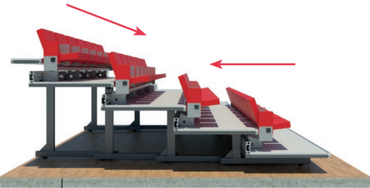
RETRACTABLE SEATING SYSTEM
