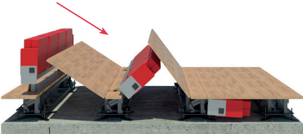
MUTASUB SEATING SYSTEM
