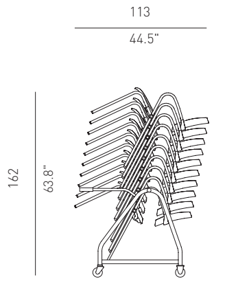
Storage Cart
